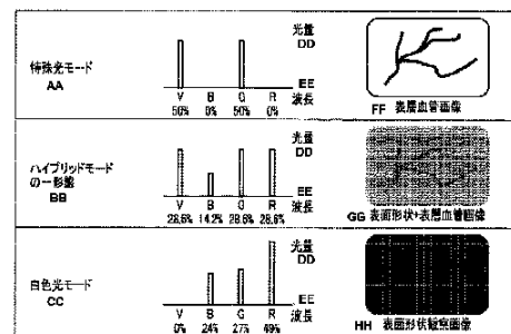
FIG. 2: AA: Special light mode BB: One form of hybrid mode CC: White light mode DD: Light amount EE: Wavelength FF: Superficial blood vessel image GG: Surface shape + superficial blood vessel image HH: Surface shape observation image
